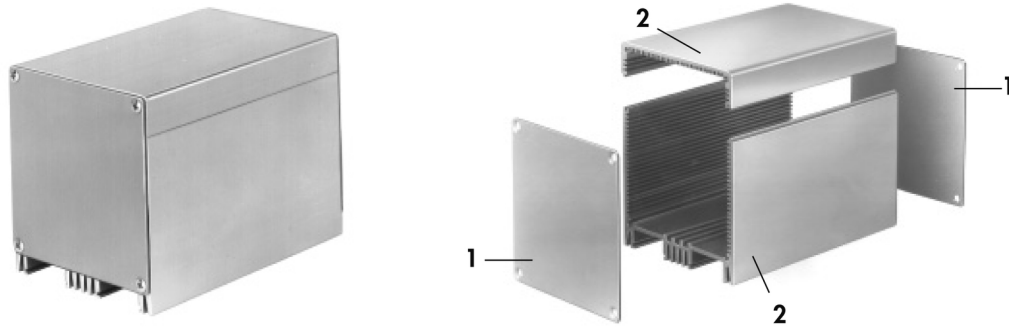
1 cover plate; 2 aluminium profile
